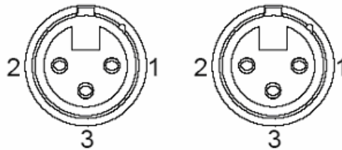
XLR 3p Female-panel Pinout
